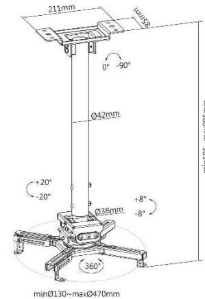
052-3011 Projector ceiling mount, black Adjustable height 60 to 90 cm
