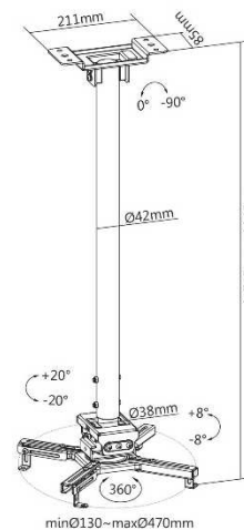
052-3021 Projector ceiling mount, black Adjustable height 75 to 115 cm
