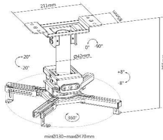
052-3021 Projector ceiling mount, black Adjustable height 75 to 115 cm
